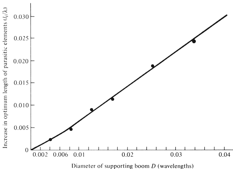
Figure 10.28 Increase in optimum length of parasitic elements as a function of metal boom diameter. (SOURCE: P. P. Vezibicke, "Yagi Antenna Design," NBS Technical Note 688, U.S. Department of Commerce/National Bureau of Standards, December 1976).
