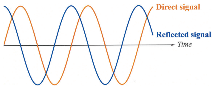
Figure 16.14 Two out-of-phase multipath signals [3].
