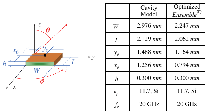
Figure 16.37 Rectangular patch antenna design using the cavity model.
