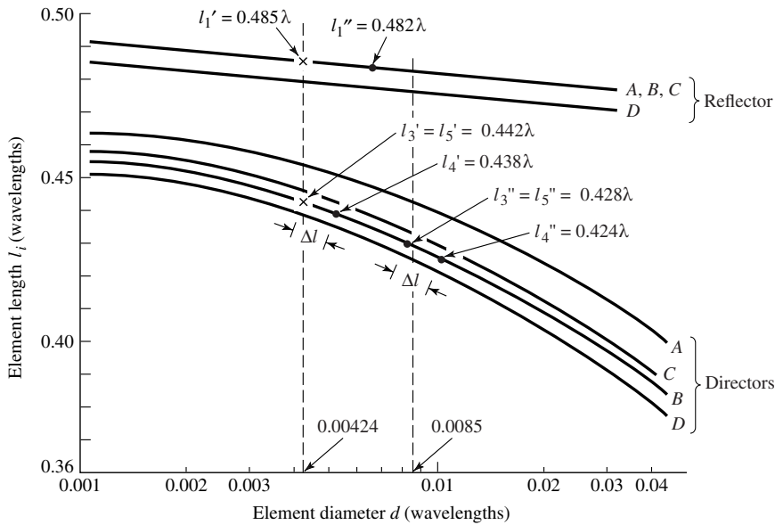
Figure 10.27 Design curves to determine element lengths of Yagi-Uda arrays. (SOURCE: P. P. Vezibicke, "Yagi Antenna Design," NBS Technical Note 688, U.S. Department of Commerce/National Bureau of Standards, December 1976).
