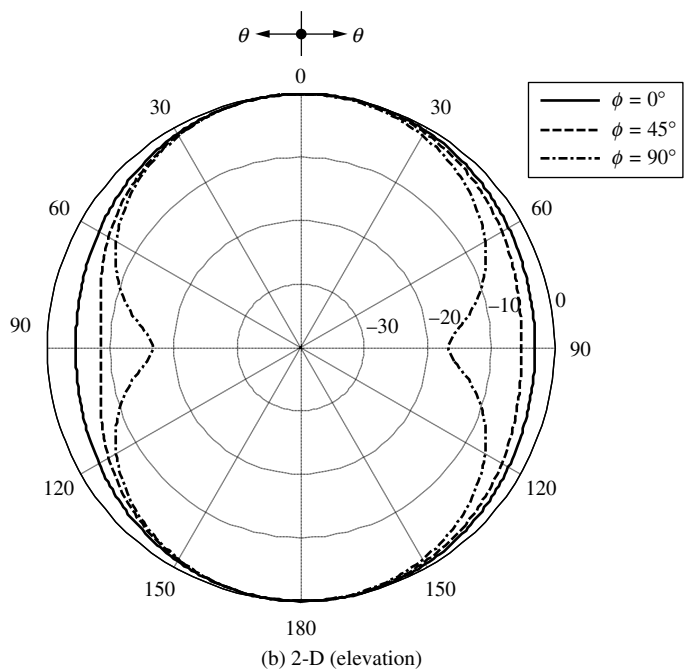
Figure 5.12 Far-field normalized three- and two-dimensional amplitude patterns for a loop with C = \lambda and \Omega = 10 .
