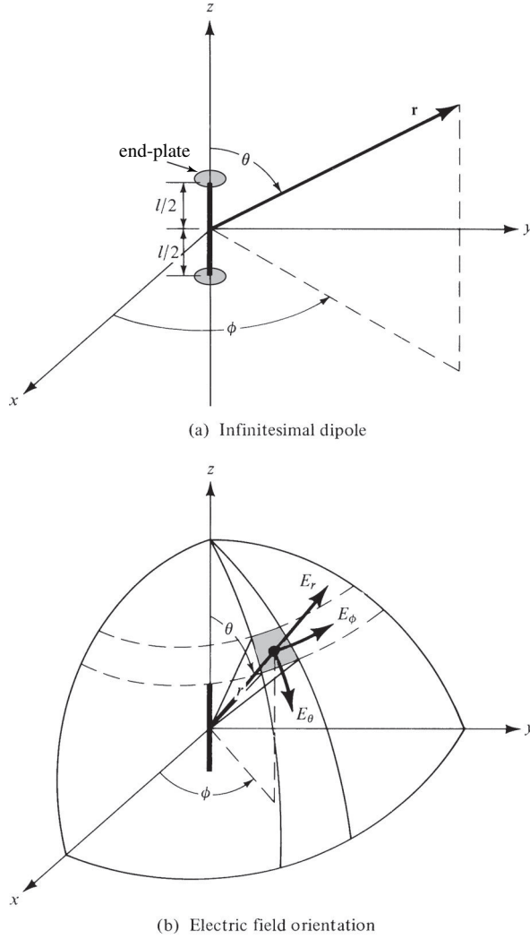
Figure 4.1 Geometrical arrangement of an infinitesimal dipole and its associated electric-field components on a spherical surface.
