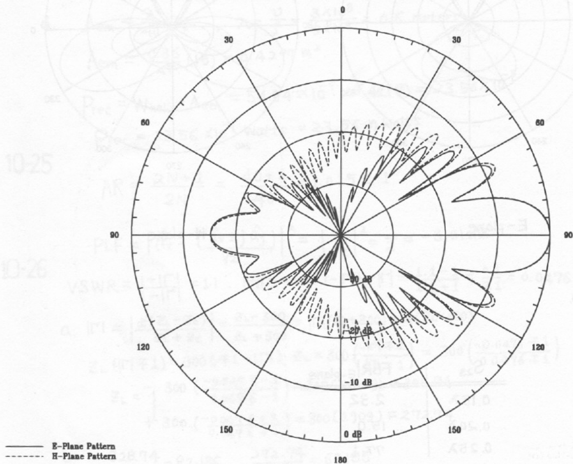
E and H Plane Field Pattern of Yagi-Uda Antenna (Prob. 10-28)
