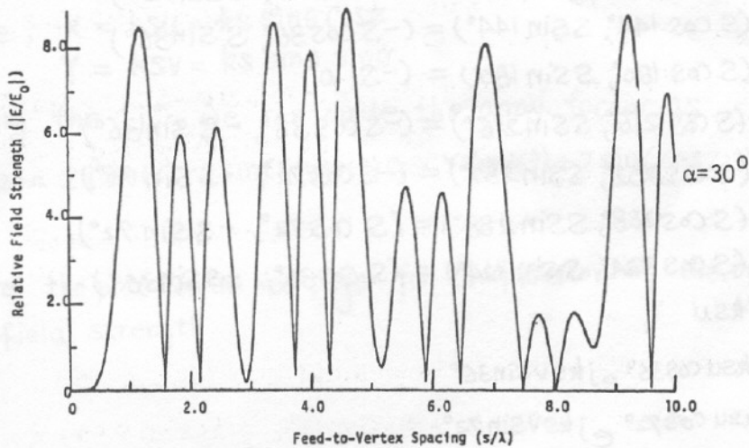
Fig. P15-2. Relative field strengths along the axis ( \theta = 90^\circ , \phi = 0^\circ ) for \alpha = 60^\circ , 45^\circ , 30^\circ corner reflectors as a function of feed-to-vertex spacing.
