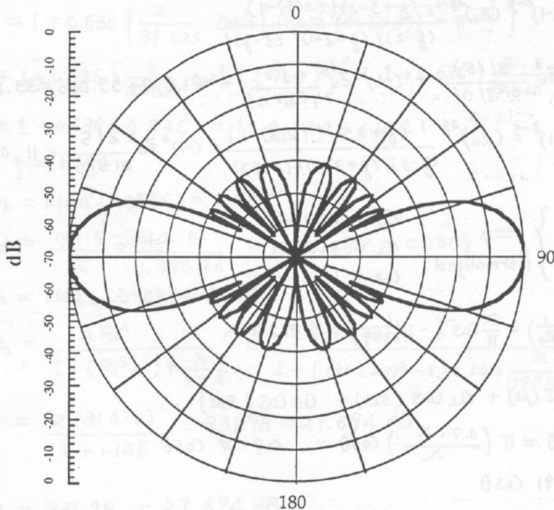
Fig. P6-45. FOUR SIDE LOBES ALL AT -40 dB LEVEL
