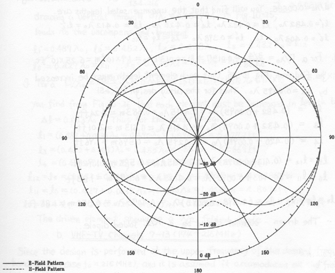
E and H Plane Field Pattern of Yagi-Uda Antenna (Prob. 10-29)
