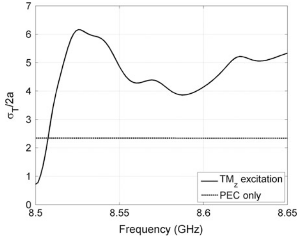
Fig. 12.14 Normalized total scattering width versus frequency for TM_z cloak with included dispersion ( TM_z polarization) [7]
