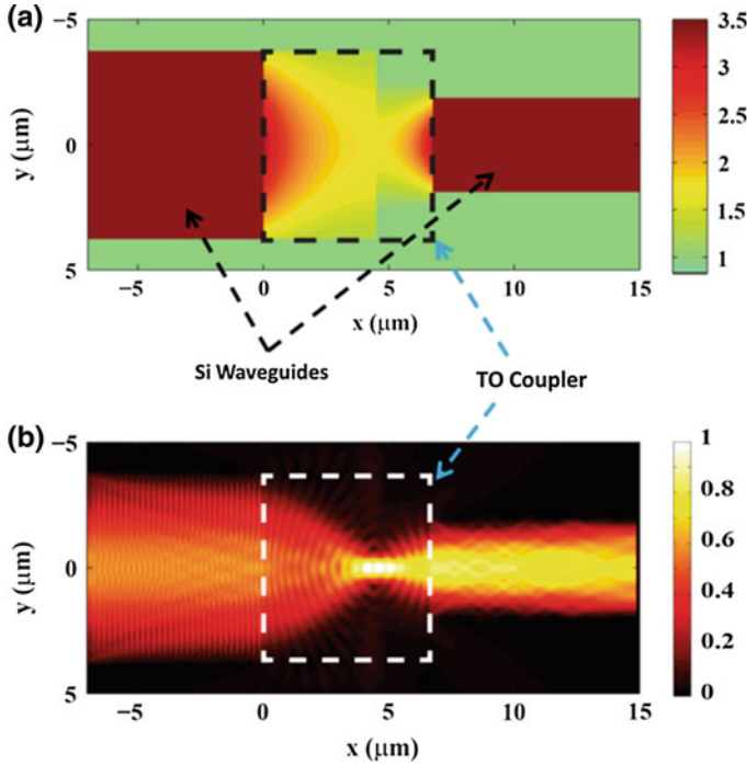
Fig. 2.34 a A TO-based GRIN waveguide coupler connects two silicon waveguides with a width of 7.5 \mu\text{m} and 3.75 \mu\text{m} , respectively. The coupler device, illustrated in the black dashed box, has a size of 7.5 \mu\text{m} by 6.7 \mu\text{m} . b Light intensity distribution obtained from FDTD simulations. Light from the input waveguide on the left couples well into the output waveguide through the TO coupler
