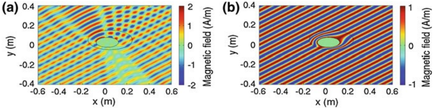
Fig. 2.4 Snapshots of the total magnetic field for a 2D eccentric elliptic annular cloak due to an elliptic conducting cylinder subject to a plane wave illumination. a Bare conducting cylinder exposed to incoming plane wave. b The same cylinder enclosed by the cloak
