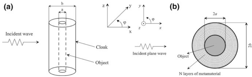
Fig. 12.2 A sketch of the anisotropic cloak. a A general case with hypothetical continuous material. b Multilayer realization
