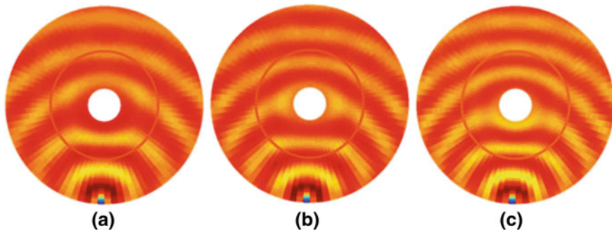
Fig. 12.38 ADS TM simulation of a cloaked conducting cylinder-design based on lumped circuits that contain ideal negative non-Foster capacitors and inductors, (the point source is located at the bottom of the computational domain; warmer colors correspond to higher node voltages). a f/f_0 = 0.9 , b f/f_0 = 1 , and c f/f_0 = 1.1
