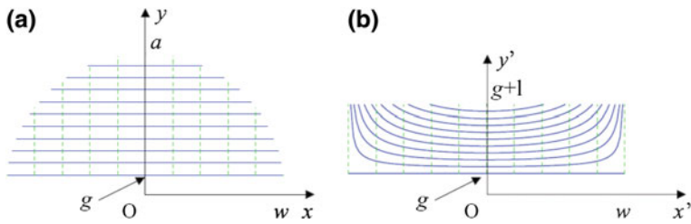
Fig. 8.20 Coordinate transformation. a Source domain and b destination domain for TO collimating lens, designed by Kwon and Werner [67]. Reproduced with permission from Kwon and Werner [67]
