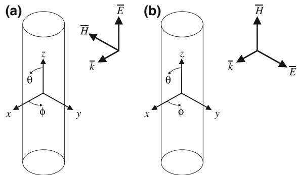
Fig. 11.1 Definitions of TE and TM incidences adopted in this Chapter, for the case of an incident wave illuminating a cylindrical scattering object. a TE incidence. b TM incidence
